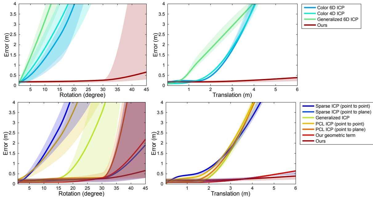
Figure 2. Evaluation of LiDAR point cloud alignment on the Cathedral scene [5]. The presented algorithm is compared to prior algorithms that use color (top) and to algorithms that do not (bottom). The algorithms are initialized with transformations that are perturbed away from the true pose in the rotational component (left) and the translational component (right). The plot shows the median RMSE at convergence (bold curve) and the 40%-60% range of RMSE across trials (shaded region). Lower is better.
