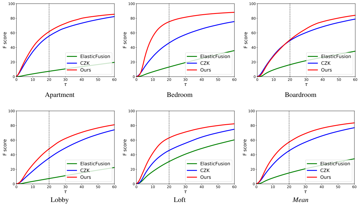
Figure 3. Accuracy of different reconstruction systems on the five scenes in the presented dataset, measured by F-score with varying distance thresholds \tau (in millimeters). The last plot shows the mean F-score for each threshold over all five scenes in the dataset.
