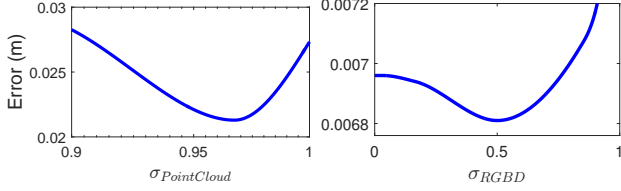
Figure 1. Grid search for \sigma in colored point cloud registration (left) and RGB-D image alignment (right).
