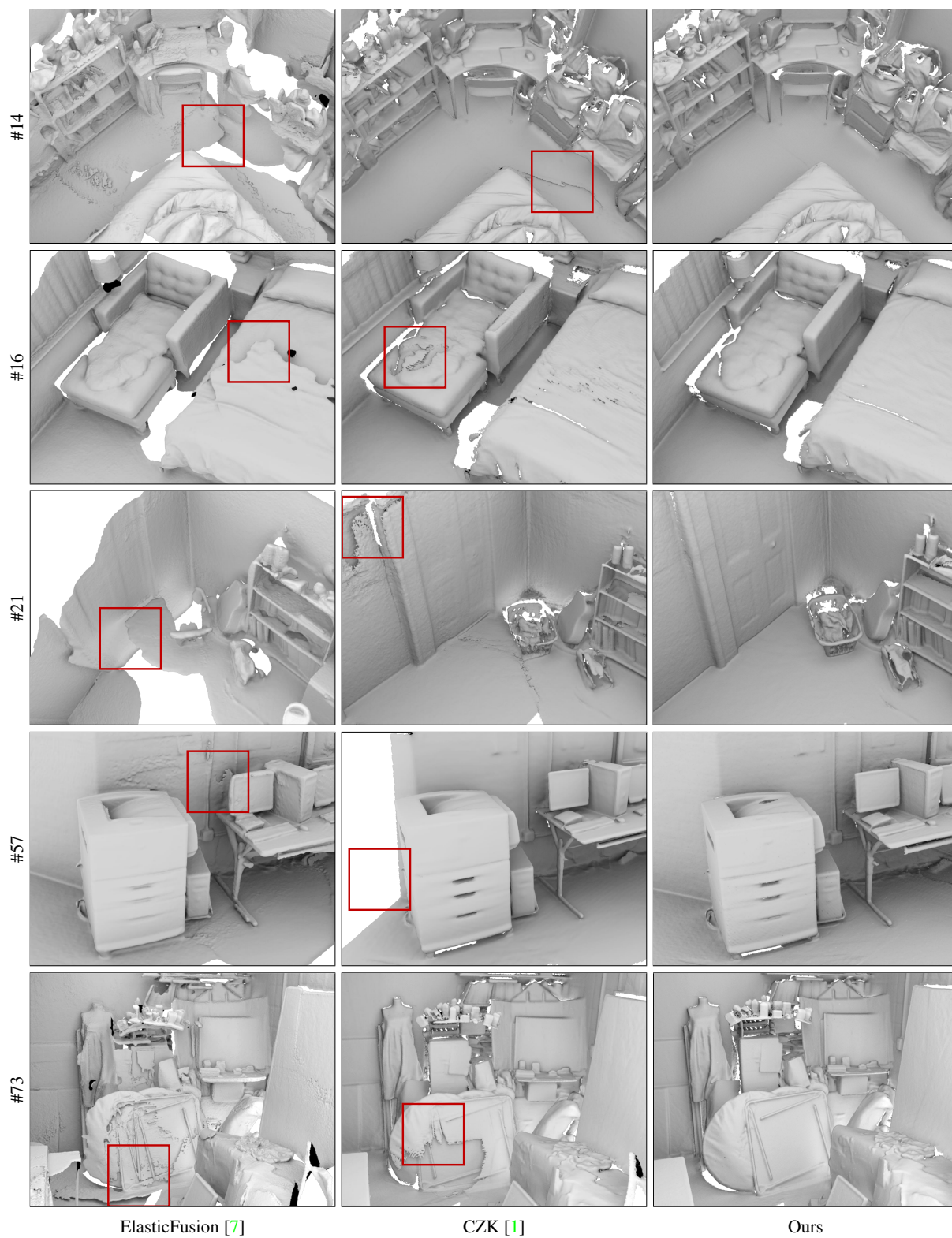
Figure 5. Reconstructions of five more scenes from the SceneNN dataset [2]. This extends Figure 4 in the paper. Prior systems suffer from inaccurate surface alignment and produce broken geometry. Our system produces much cleaner results.
